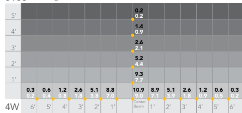
5106 4W Integrated LED
